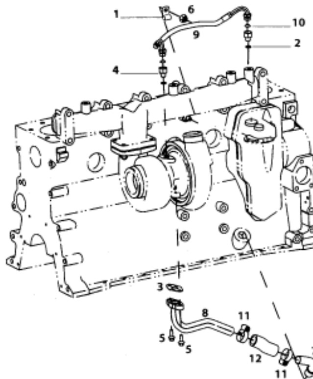
TURBOCHARGER PLUMBING (BS I)
