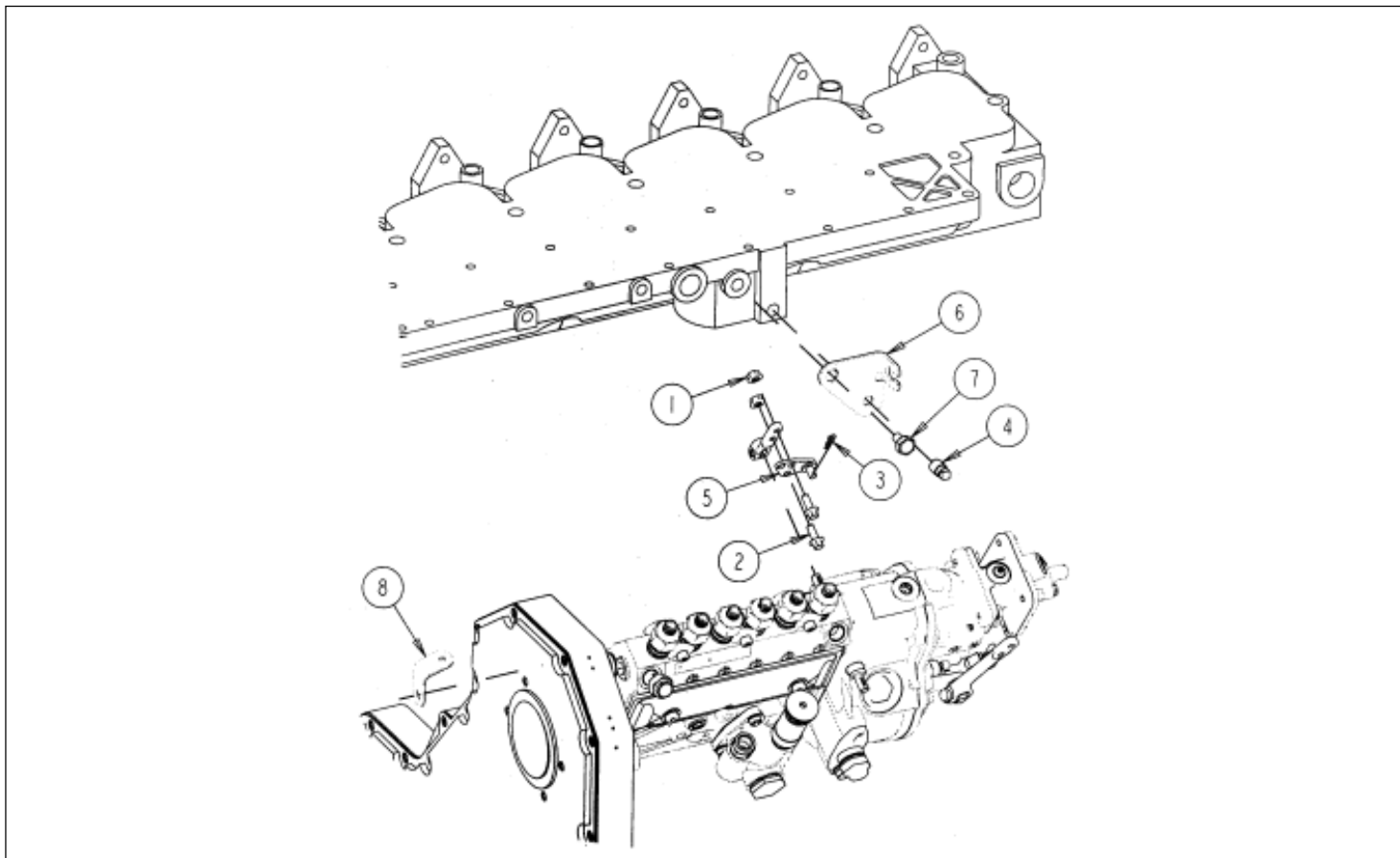
LEVER, FUEL SHUTOFF
