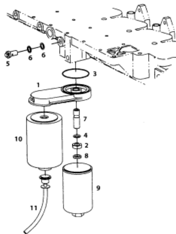
FUEL FILTER (BS I)
