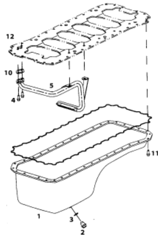
OIL PAN
