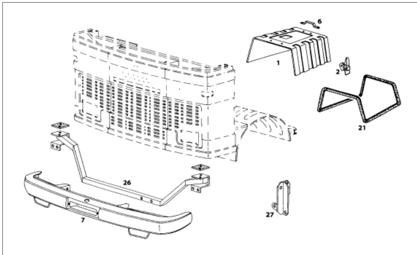
BUMPER, ENGINE HOOD AND ANTI SAGGING BAR
