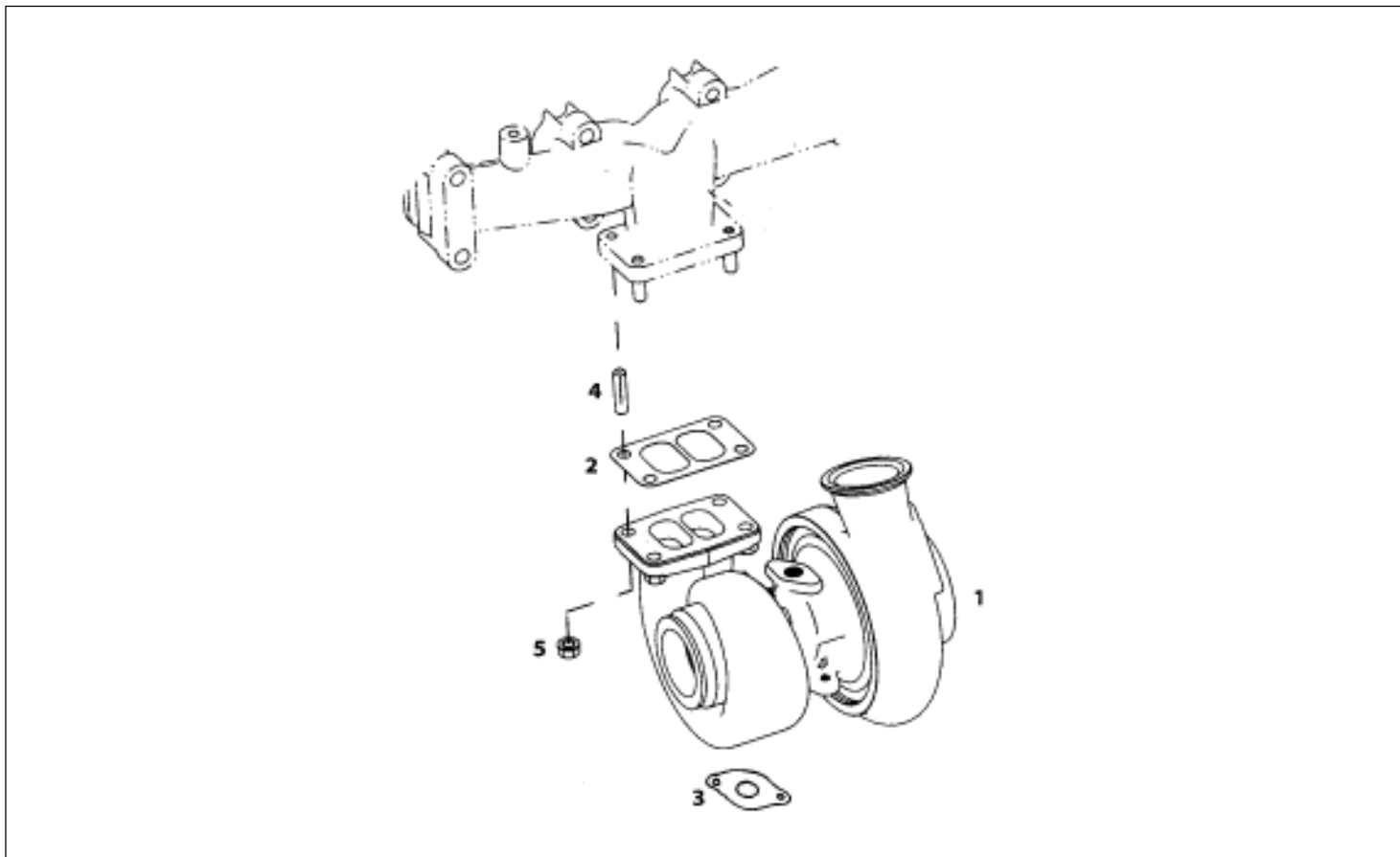
TURBOCHARGER (LOW MOUNT) (BS I)
